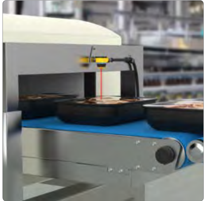
Detection in a washdown environment using a T18-2
