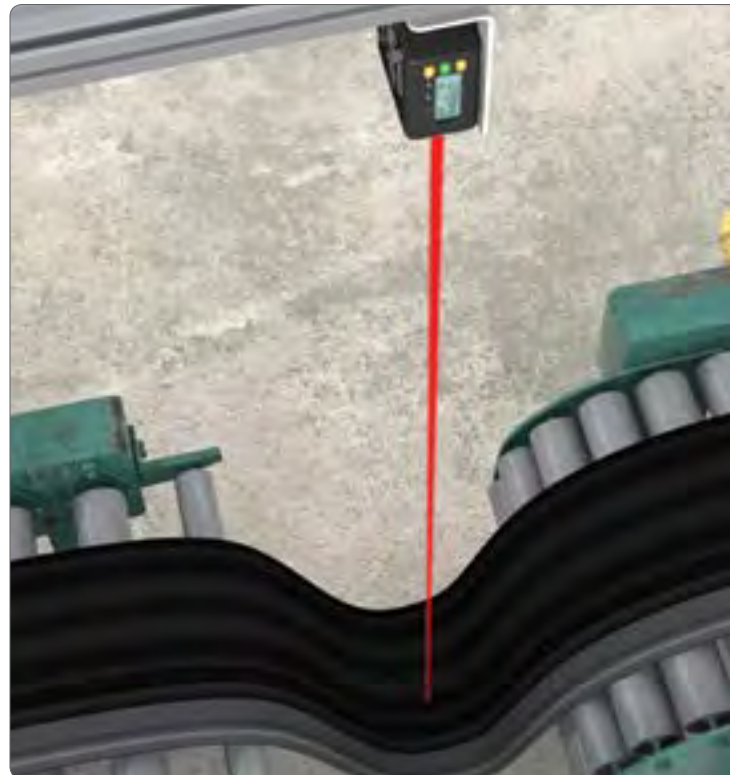
Loop control on a calendering machine
